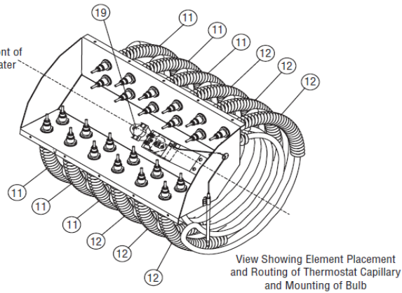
Element Assembly 60kW
