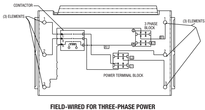
Figure 3b. Wiring Connections for Single-Phase and Three-Phase Power (HUHAA724FC, HUHAA1020FC, HUHAA1024FC)
