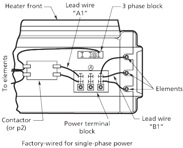
Figure 3a. Wiring Connections for Single-Phase and Three-Phase Power (HUHAA520FC, HUHAA524FC, HUHAA720FC)
