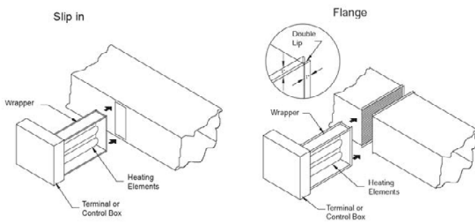
Drawing 1: Slip in and flange frame types
